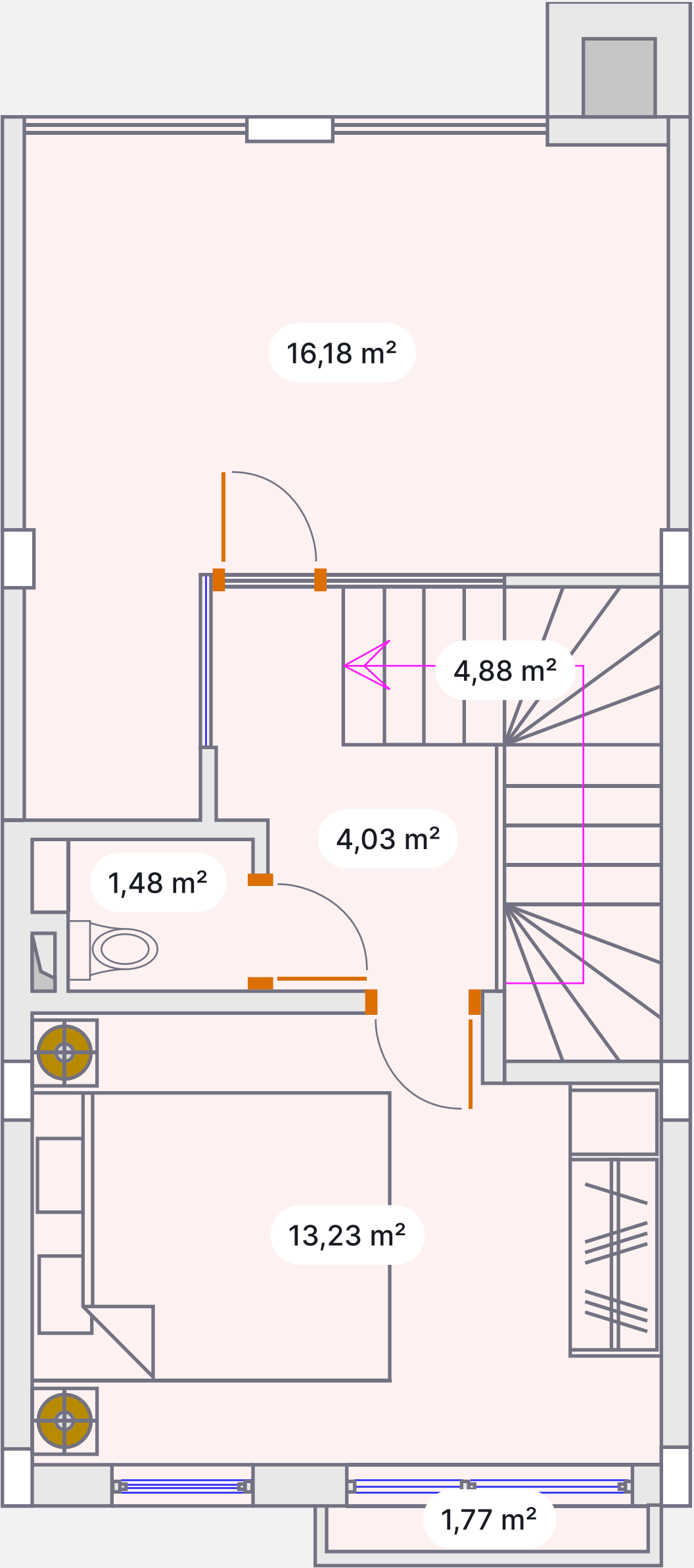
3rd floor
